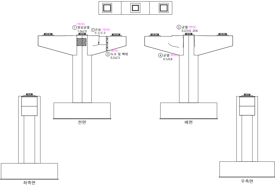
KEY PLAN
