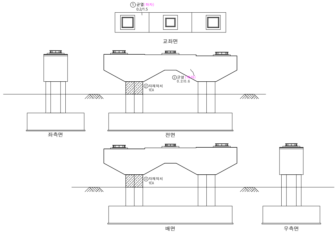
SECTION
